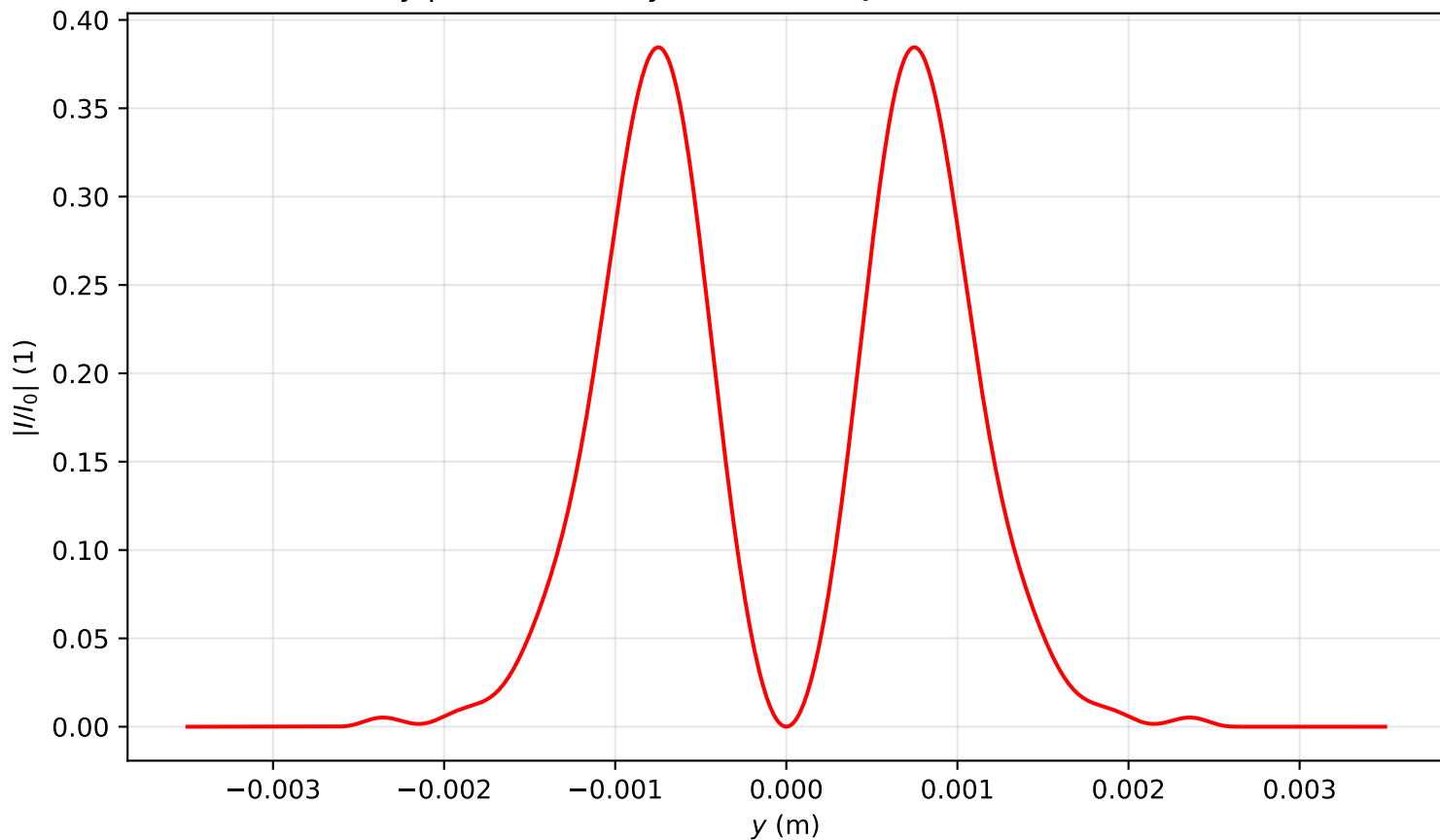
Intensity profile I(x=0, y, z=2.866)/I_0 , \text{Pin}=3.0\text{Pcr} , artificial time
